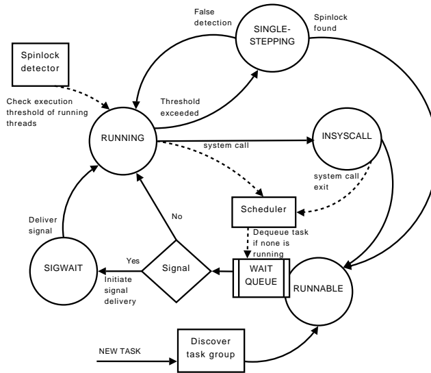
Figure 5.3: Scheduler FSM
