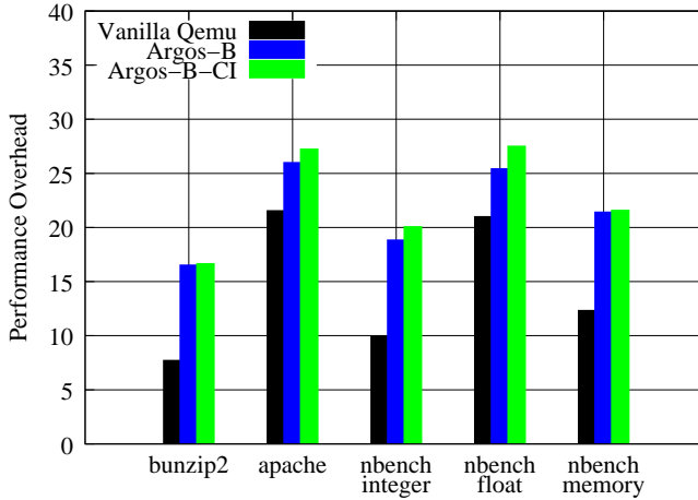
Figure 3.5: Performance Benchmarks
